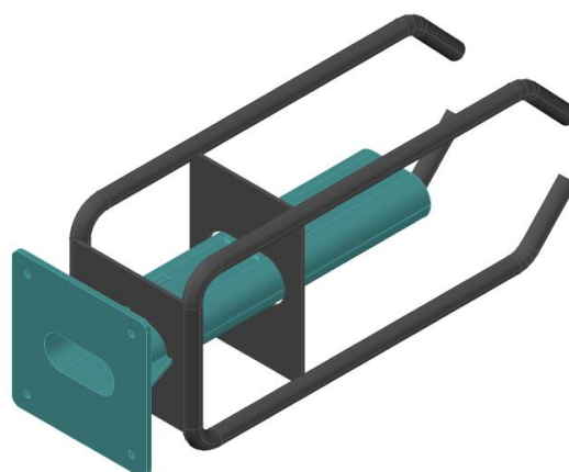
Figure A2.5: Female component with polypropylene sleeve for axial and lateral transverse movement.
