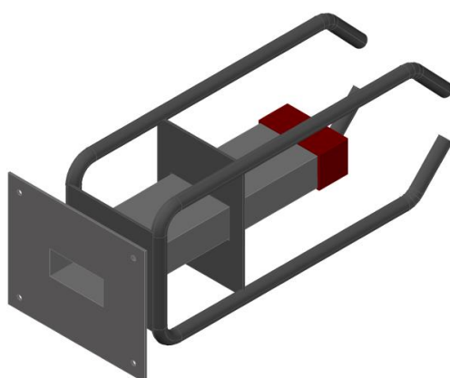
Figure A2.4: Female component with stainless steel sleeve for axial and lateral transverse movement.
