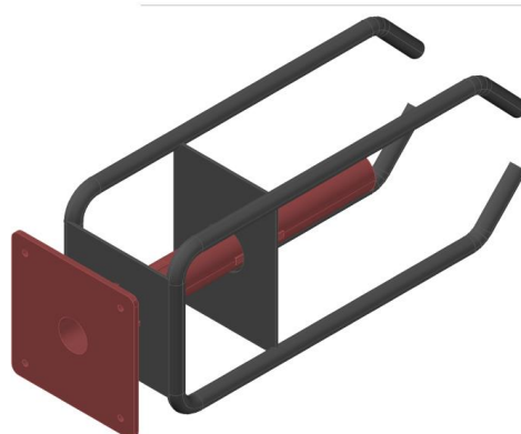
Figure A2.3: Female component with polypropylene sleeve for axial movement only.
